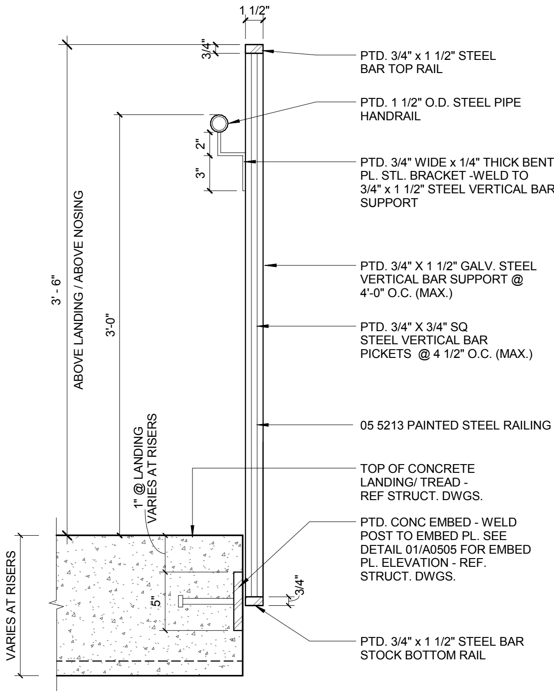
2 TYP. RAILING DTL. @ STAIR & INT. LANDING 1 1/2" = 1'-0"
